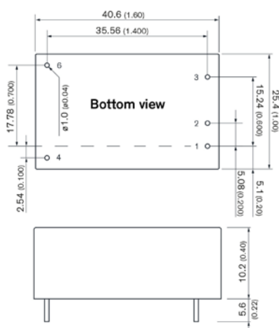
Pinout
